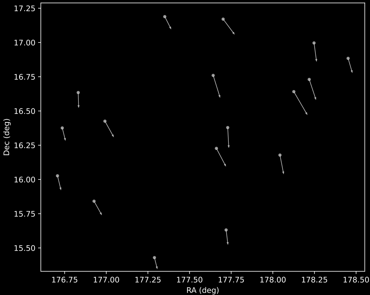
GALAH DR4 Cluster 15 Proper Motion Vectors (n=17)
