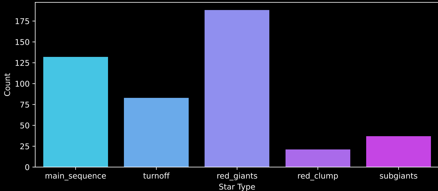
GALAH DR4 Field: [6776] Count plot of Star Type
