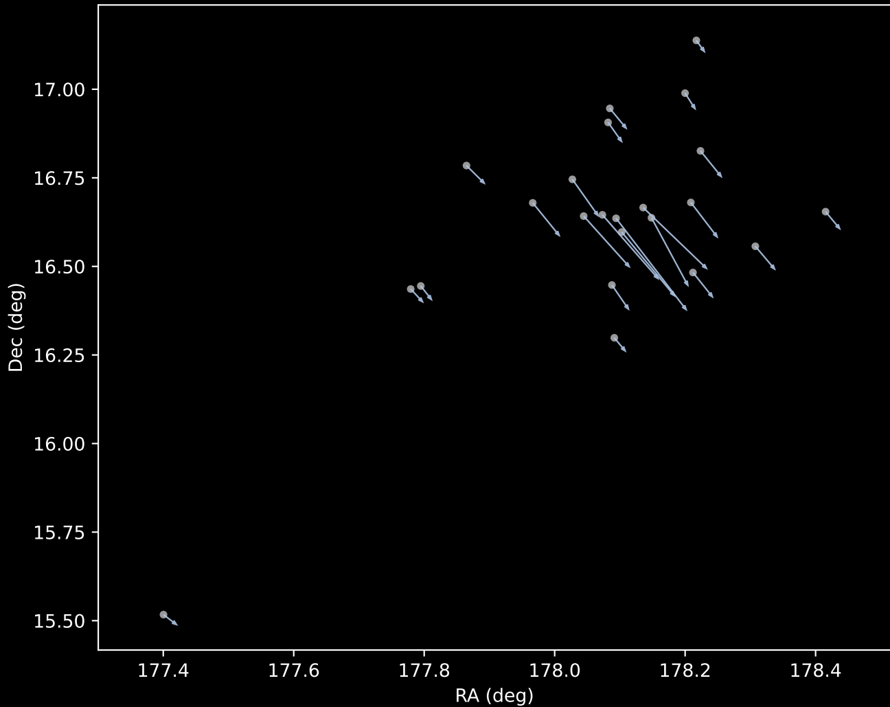
GALAH DR4 Cluster 21 Proper Motion Vectors (n=23)
